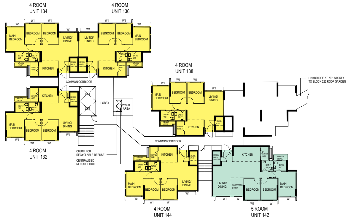
BLOCK 223A (7TH STOREY PLAN)
