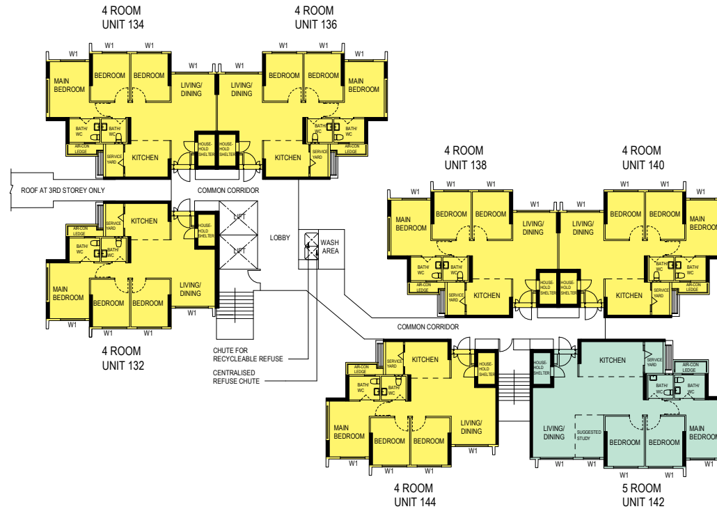
BLOCK 223A (3RD TO 6TH AND 8TH TO 11TH STOREY FLOOR PLAN)
