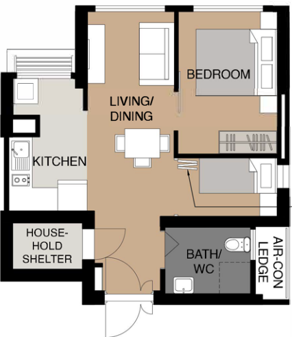
2-ROOM FLEXI (TYPE 2) FLOOR PLAN (With Suggested Furniture Layout) APPROX. FLOOR AREA 48 sqm (Inclusive of Internal Floor Area of 46 sqm and Air-Con Ledge)
