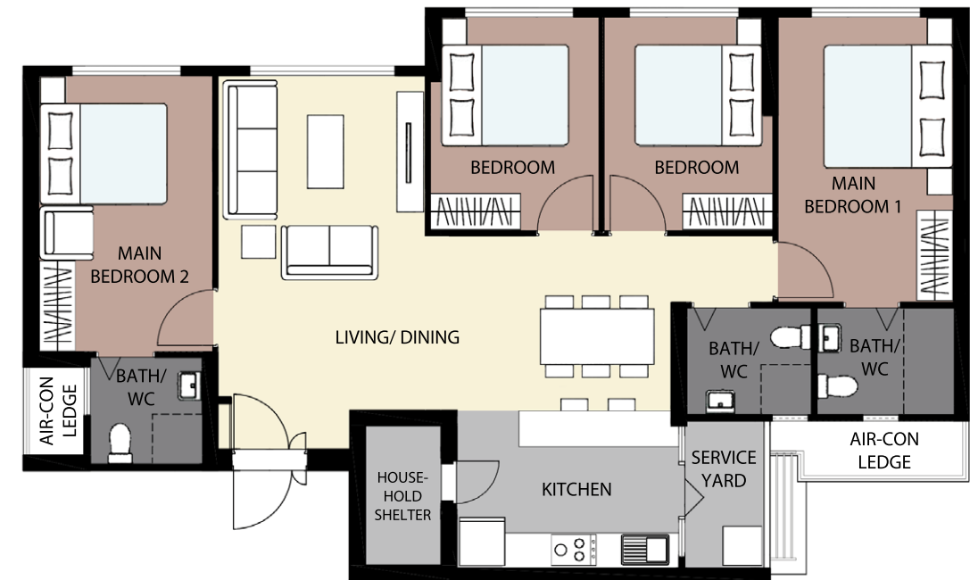
3GEN FLAT FLOOR PLAN (With Suggested Furniture Layout) APPROX. FLOOR AREA 120 sqm (Inclusive of Internal Floor Area of 115 sqm and Air-con Ledge)
