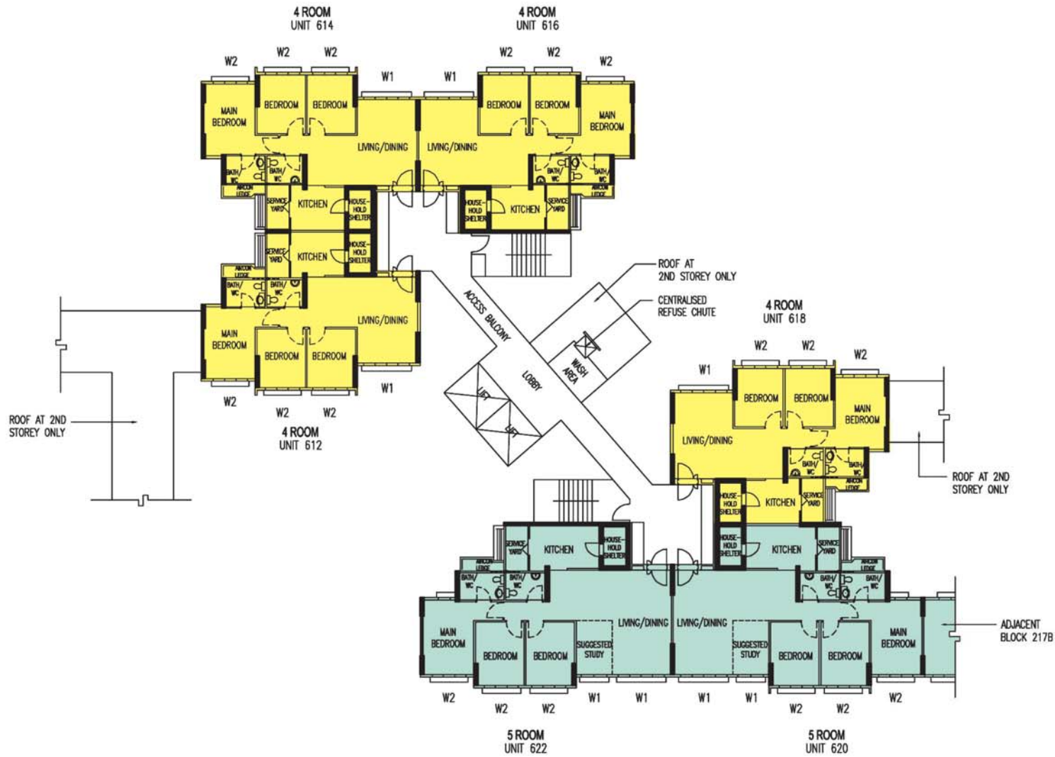
BLOCK - 217A (2ND TO 16TH STOREY FLOOR PLAN)
