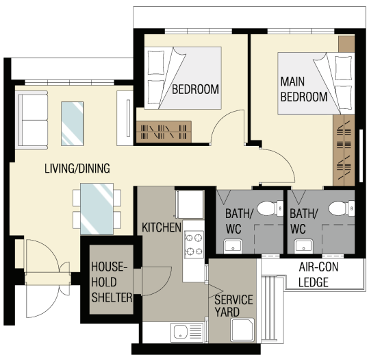
LAYOUT IDEAS FOR 3-ROOM APPROX. FLOOR AREA 69 sqm (Inclusive of Internal Floor Area 66 sqm and Air-Con Ledge)
