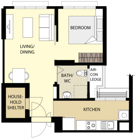
LAYOUT IDEAS FOR 2-ROOM FLEXI (TYPE 2) Approx. Floor Area of 47 sqm (Inclusive of Internal Floor Area of 45sqm and Aircon Ledge)
