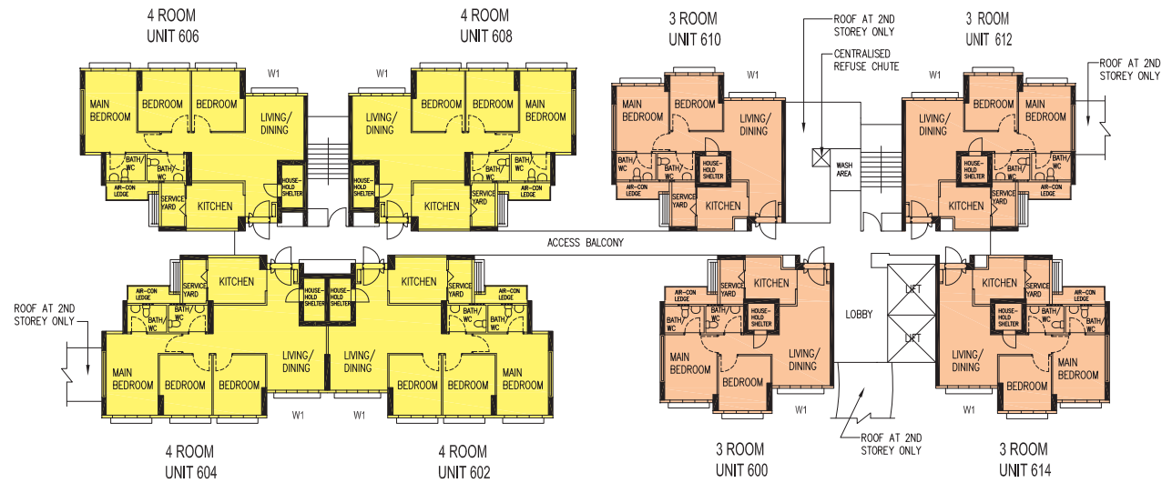
BLOCK 671A (2ND TO 13TH STOREY FLOOR PLAN)
